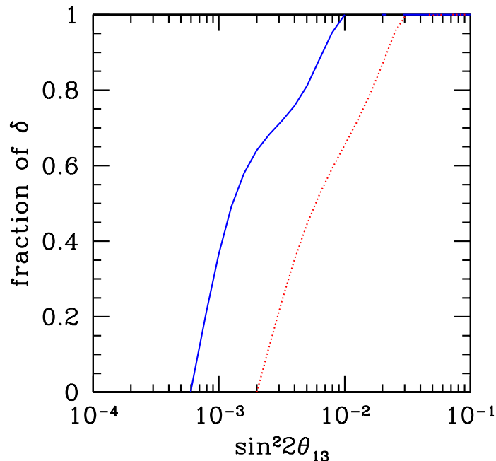
Figure 3: 99% CL hierarchy resolution (2 d.o.f). The dotted red curve depicts the results assuming an exposure of 10^{21} ion-kton-years in Boulby. The solid blue curve depicts the results assuming the statistics quoted before is improved by a factor of five.
