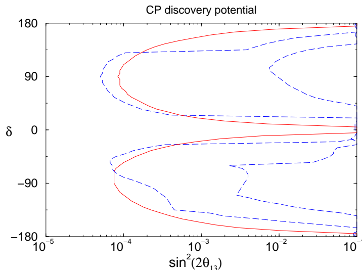
Figure 4: Discovery at 99% CL of CP violation (2 d.o.f). The dashed blue curves depict the results assuming an exposure of 10^{21} ions-kton-years and 5 \times 10^{21} ions-kton-years in Boulby. The solid red curve depicts the results for an exposure of 2.5 \times 10^{21} ions-kton-years for neutrinos and for antineutrinos, so that the total exposure is 5 \times 10^{21} ions-kton-years.
