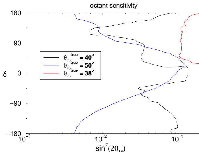
Figure 5: 99% CL determination of the \theta_{23} octant for three different true values, \theta_{23}^{\text{true}} = 38^\circ, 40^\circ and 50^\circ . The region to the right of the curves denotes the parameter space for which the octant degeneracy is not resolved at the 99% CL. Results are shown for an exposure of 5 \times 10^{21} ions-kton-years.
