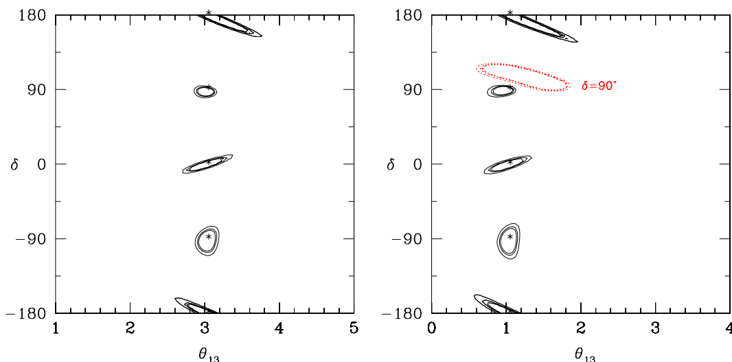
Figure 2: For an exposure of 5 \times 10^{21} ions-kton-years, 90%, 95% and 99% (for 2 d.o.f) CL contours resulting from the fits if the true values Nature has chosen are \theta_{13} = 3^\circ (left panel) or \theta_{13} = 1^\circ (right panel), and \delta = 0^\circ, 90^\circ, -90^\circ or 180^\circ . Dashed-red contours represent the \Delta\chi^2 of the hierarchy-clone solution with respect to true solution. The true solution to which the clone solution corresponds to is also shown.
